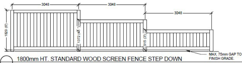
1800mm HT. STANDARD WOOD SCREEN FENCE STEP DOWN SCALE: 1:75
