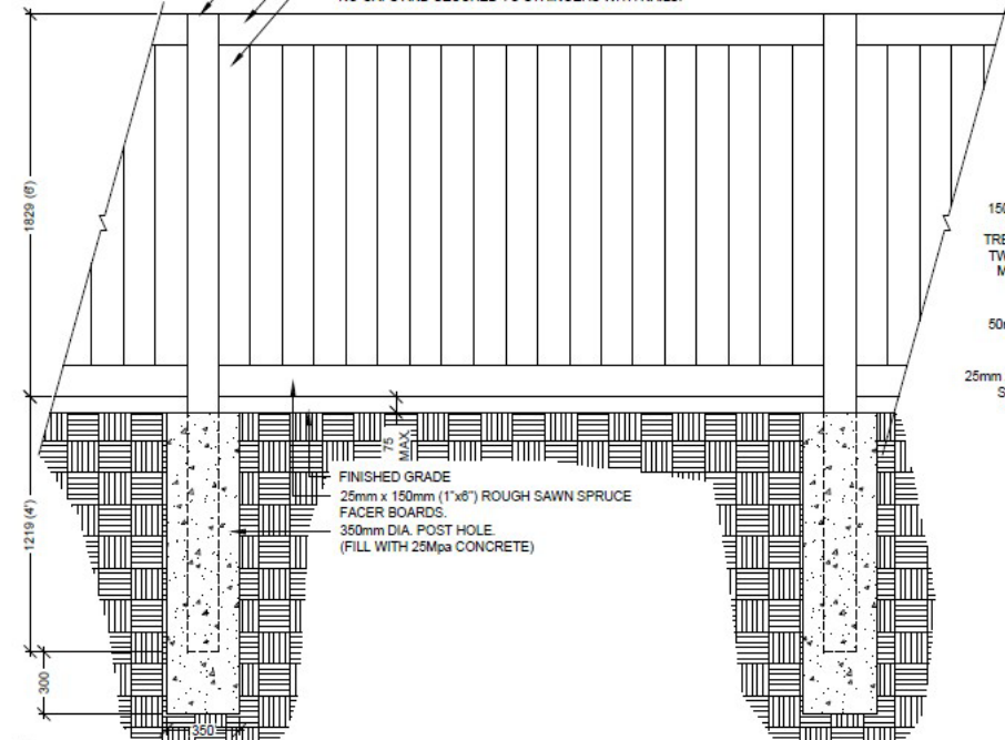
1800mm HT. STANDARD WOOD SCREEN FENCE SCALE: 1:30
